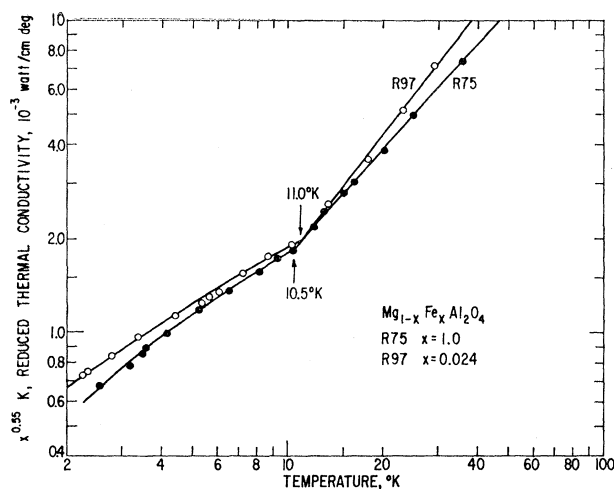
FIG. 4. The reduced thermal conductivity versus temperature in the region of 10°K. The similarity of the "kink" at 11°K for R75 and R97 is quite plain.
